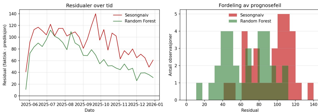
Figur 6.4: Residualanalyse
